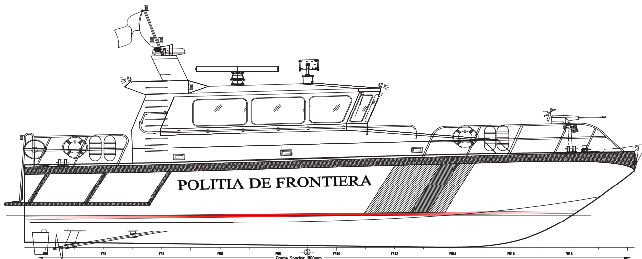
PROFILE VIEW
