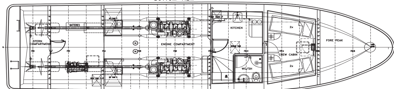
BOTTOM VIEW
